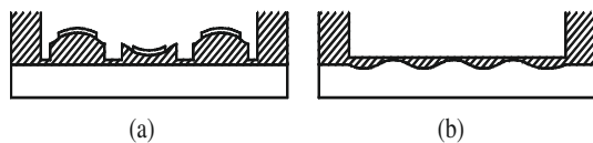
Fig. 3. Peristaltic micro-pumps. (a) Discrete geometry and (b) continuous geometry.
