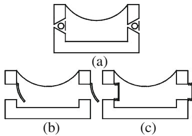
Fig. 2. Check valves. (a) Ball, (b) flap and (c) bridge.
