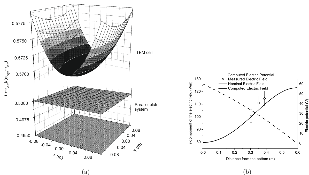
Fig. 2. Normalized electric potential distribution over a square surface around the system center in the parallel plates and in the TEM cell (a). Potential and electric field distribution along a line between the electrodes in the center of the TEM cell (b). The nominal electric field value is 100 V/m; the dots are the measured field values.
